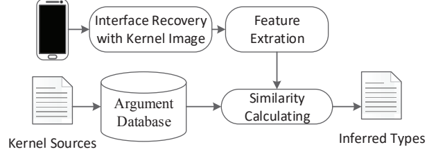
Fig. 5. The process of type inference
